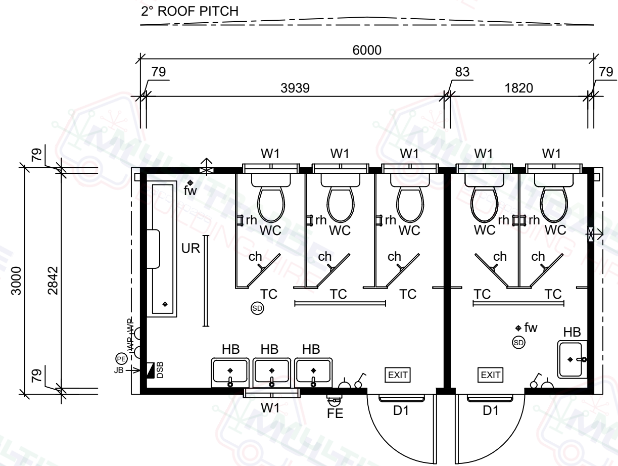
6.0x3.0m Male / Female Toilet - Floor Plan
